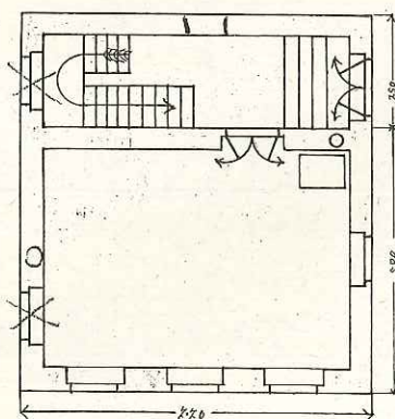
PIANTA I PIANO
